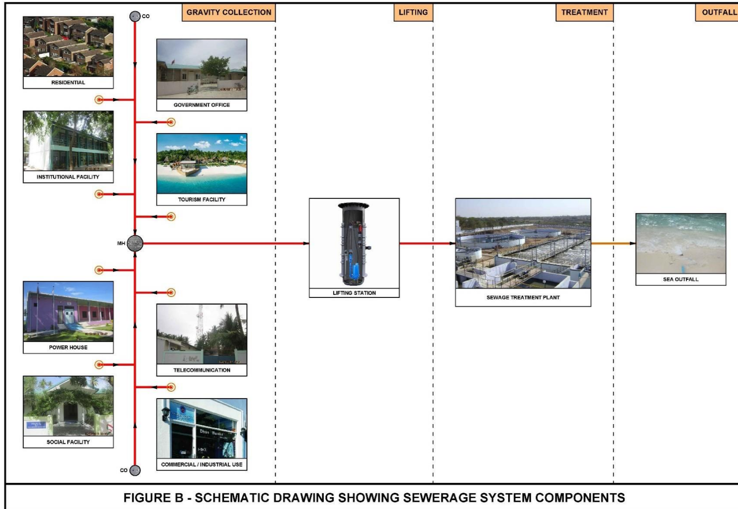
Figure 10 - Sewerage System Components
