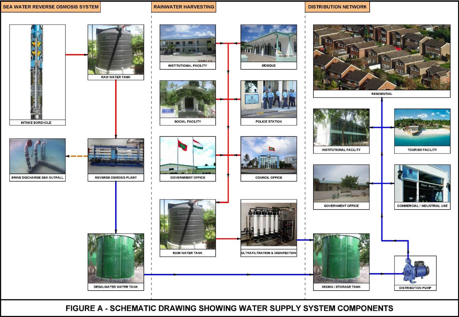
Figure 9 - Water Supply System Components
